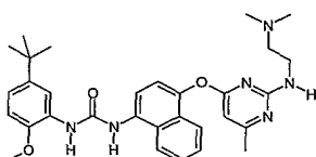
1-(5-tert-Butyl-2-methoxy-phenyl)-3-{4-[2-(2-dimethylamino-ethylamino)-6-methyl-pyrimidin-4-yloxy]-naphthalen-1-yl}-urea;
